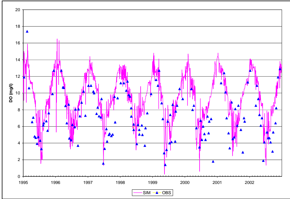
Figure B.3. Time Series of Observed and Simulated DO, Calibration Scenario, ANA01
