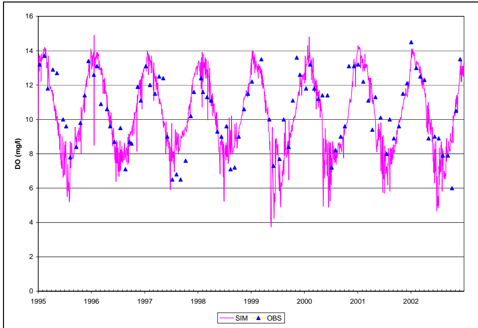
Figure B.1. Time Series of Observed and Simulated DO, Calibration Scenario, ANA0082
